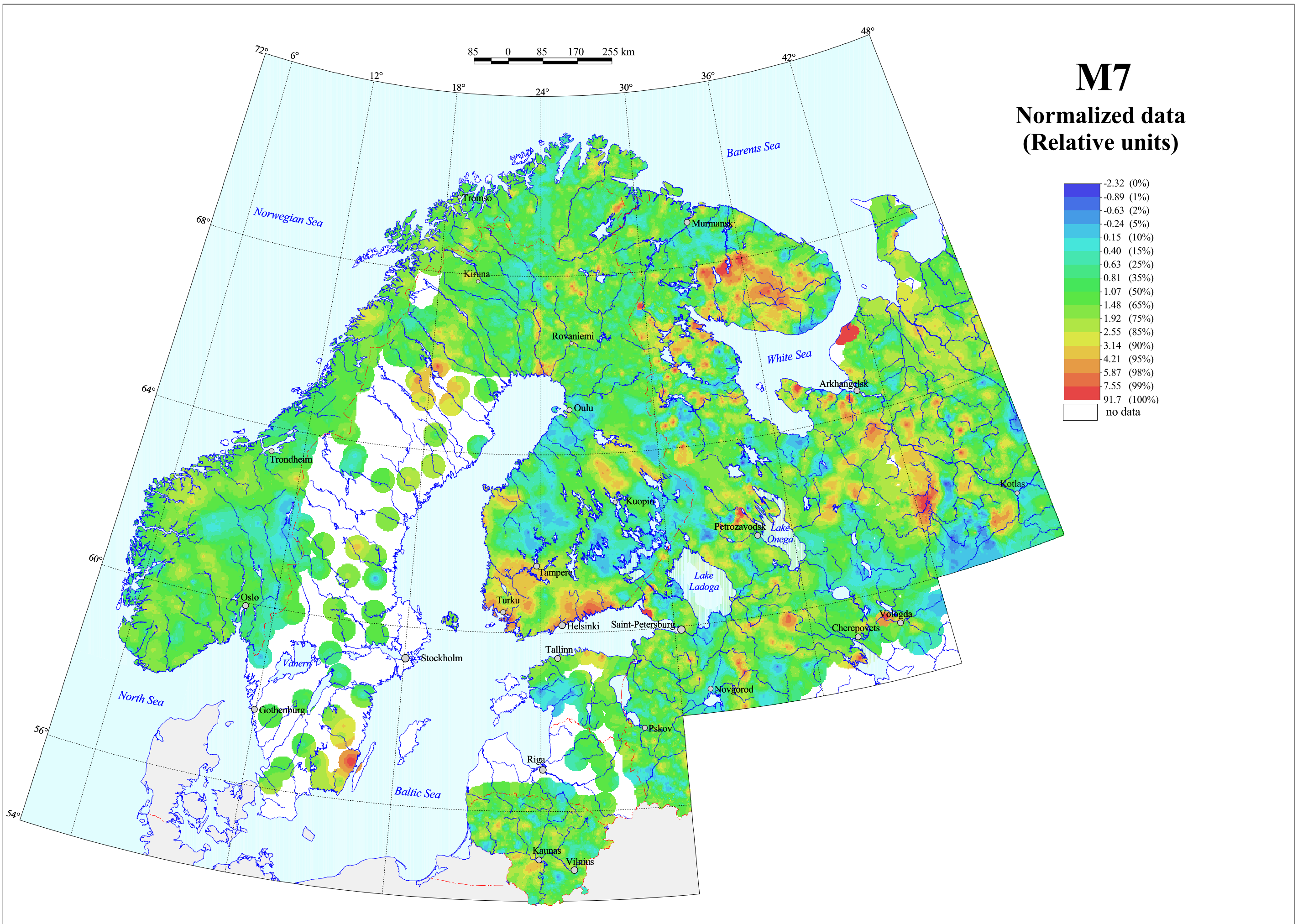
M7 (Be, Zr, Ti, Sc) in Stream Sediment
